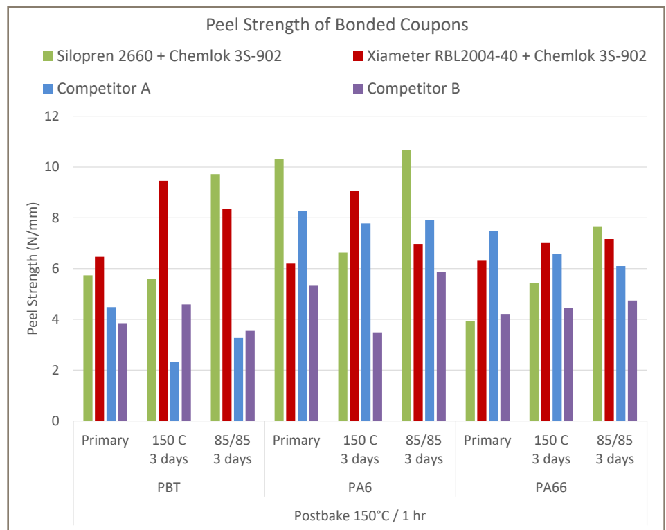
Figure 2: Average peel strength of LSR modified with Chemlok 3S-902 additive, bonded to various plastics, compared to commercially available self-bonding grades. Coupons were postbaked.
